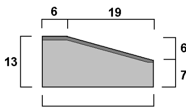
BORDILLO REMONTABLE
